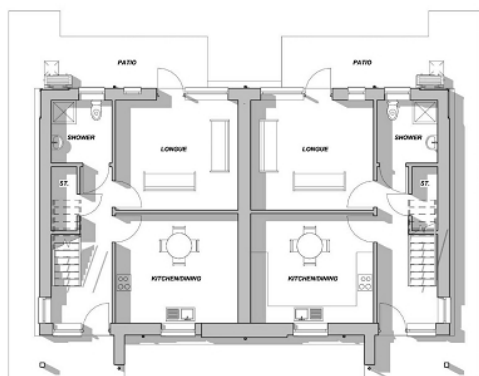
Ground floor 1 : 100
