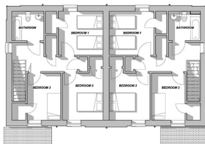
First floor 1 : 100
